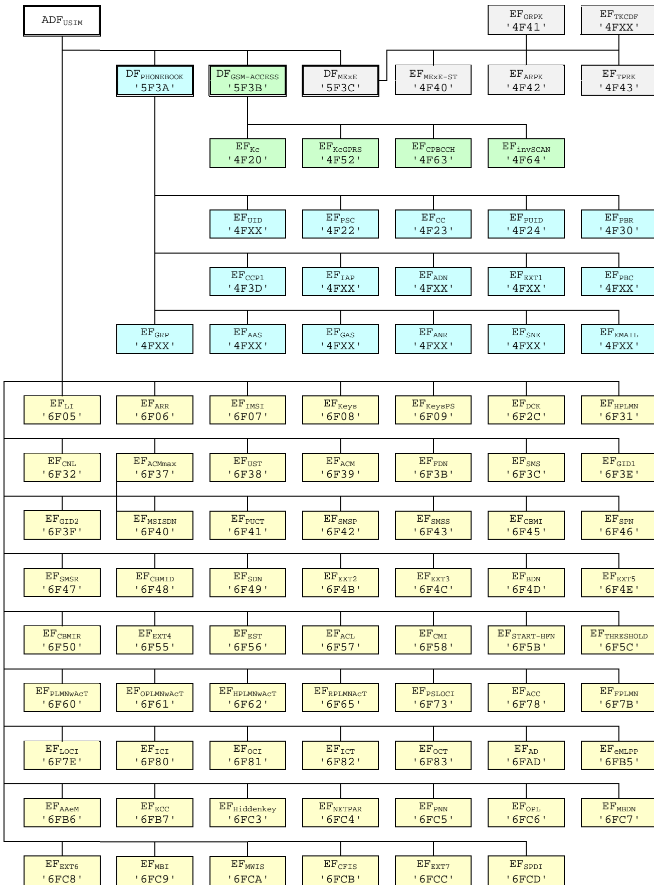
Figure 4.2: File identifiers and directory structures of USIM
