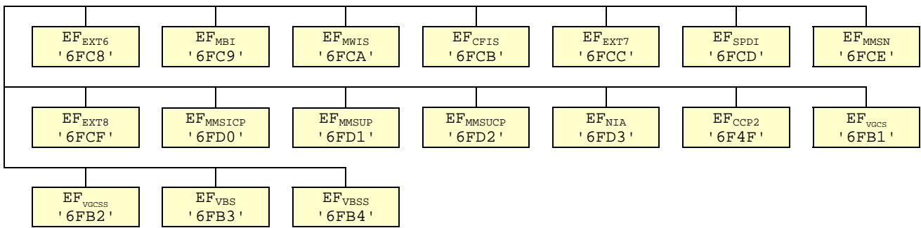
Figure 4.2: File identifiers and directory structures of USIM
