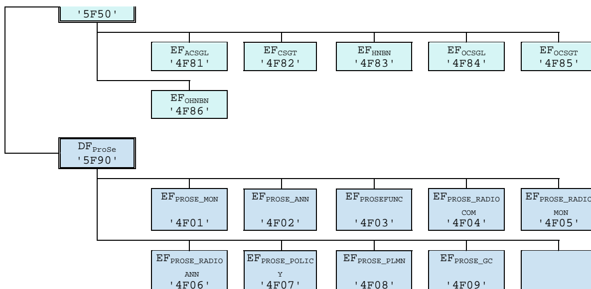
Figure 4.2: File identifiers and directory structures of USIM
