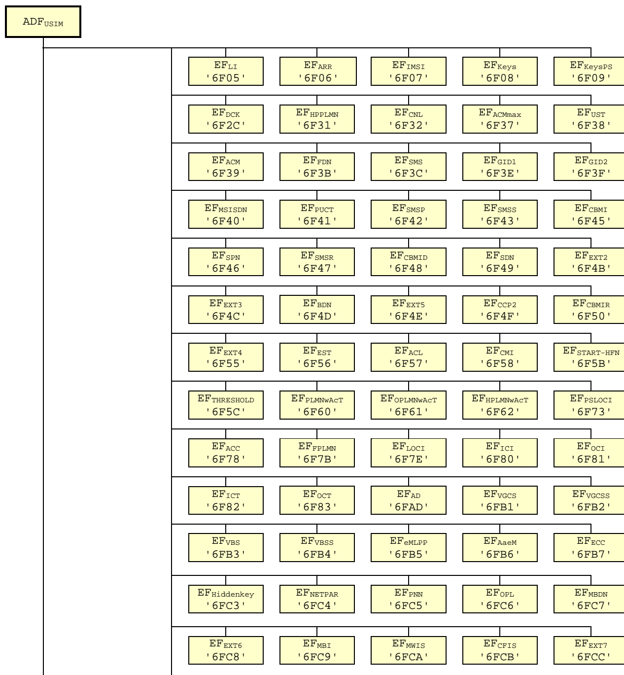
Figure 4.1: File identifiers and directory structures of UICC
