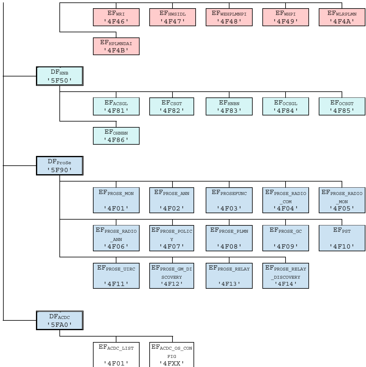
Figure 4.2: File identifiers and directory structures of USIM
