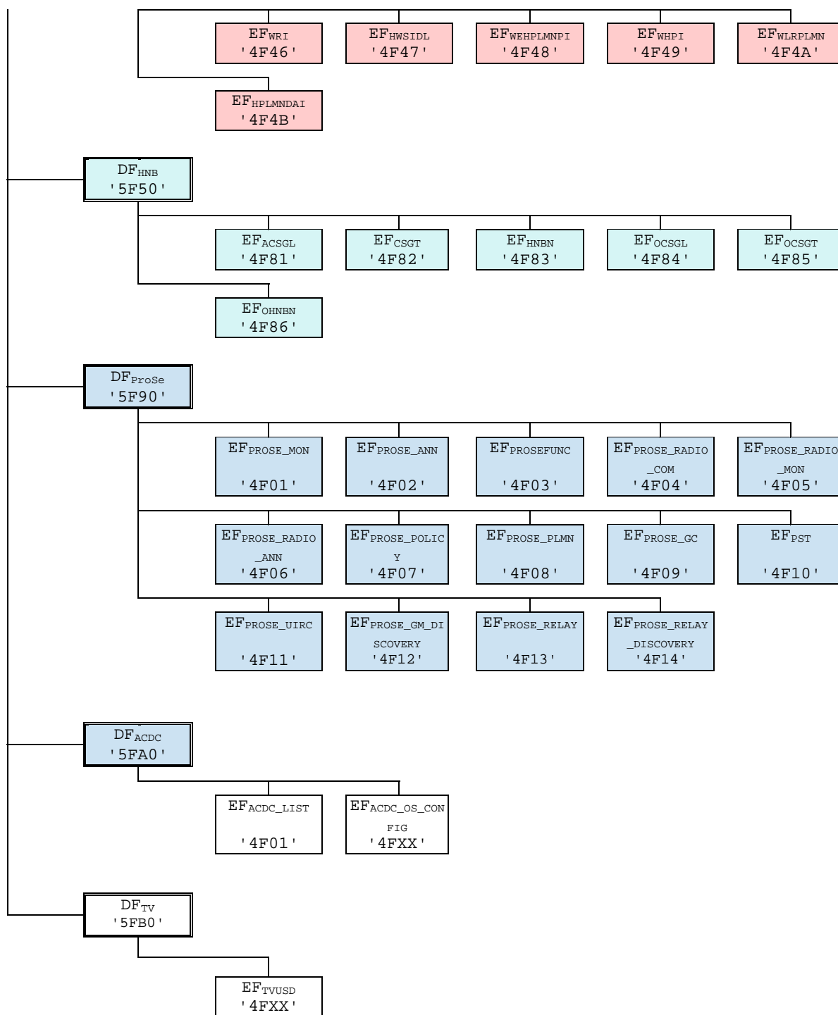
Figure 4.2: File identifiers and directory structures of USIM
