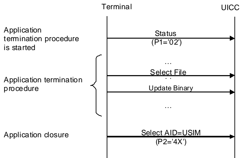
Figure I.2 USIM Application Session Termination procedure
