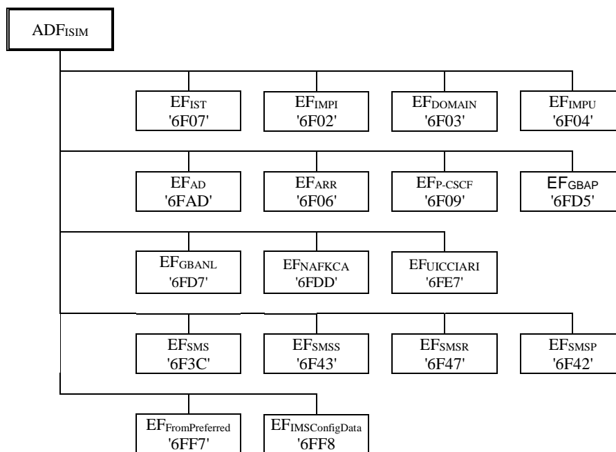
Figure 1: File identifiers and directory structures of ISIM
