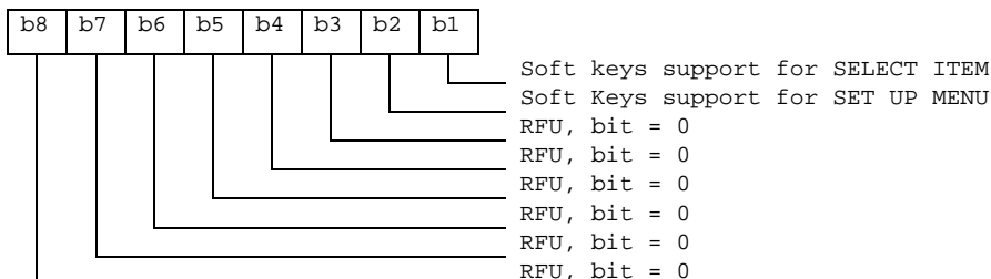
Eleventh byte: (Soft keys information)
