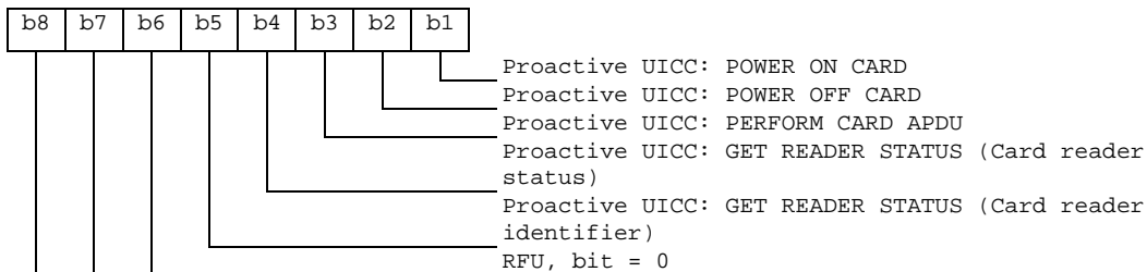
Eighth byte (Proactive UICC):
