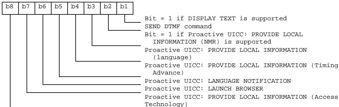
Tenth byte (Soft keys support) for class "d":
