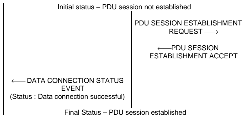
Figure T.2.3 Successful PDU session establishment procedure
