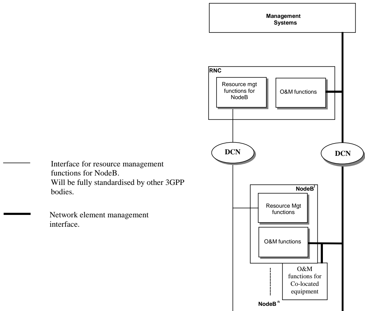
Figure 8.2: Network and Subnetwork Management Architecture
