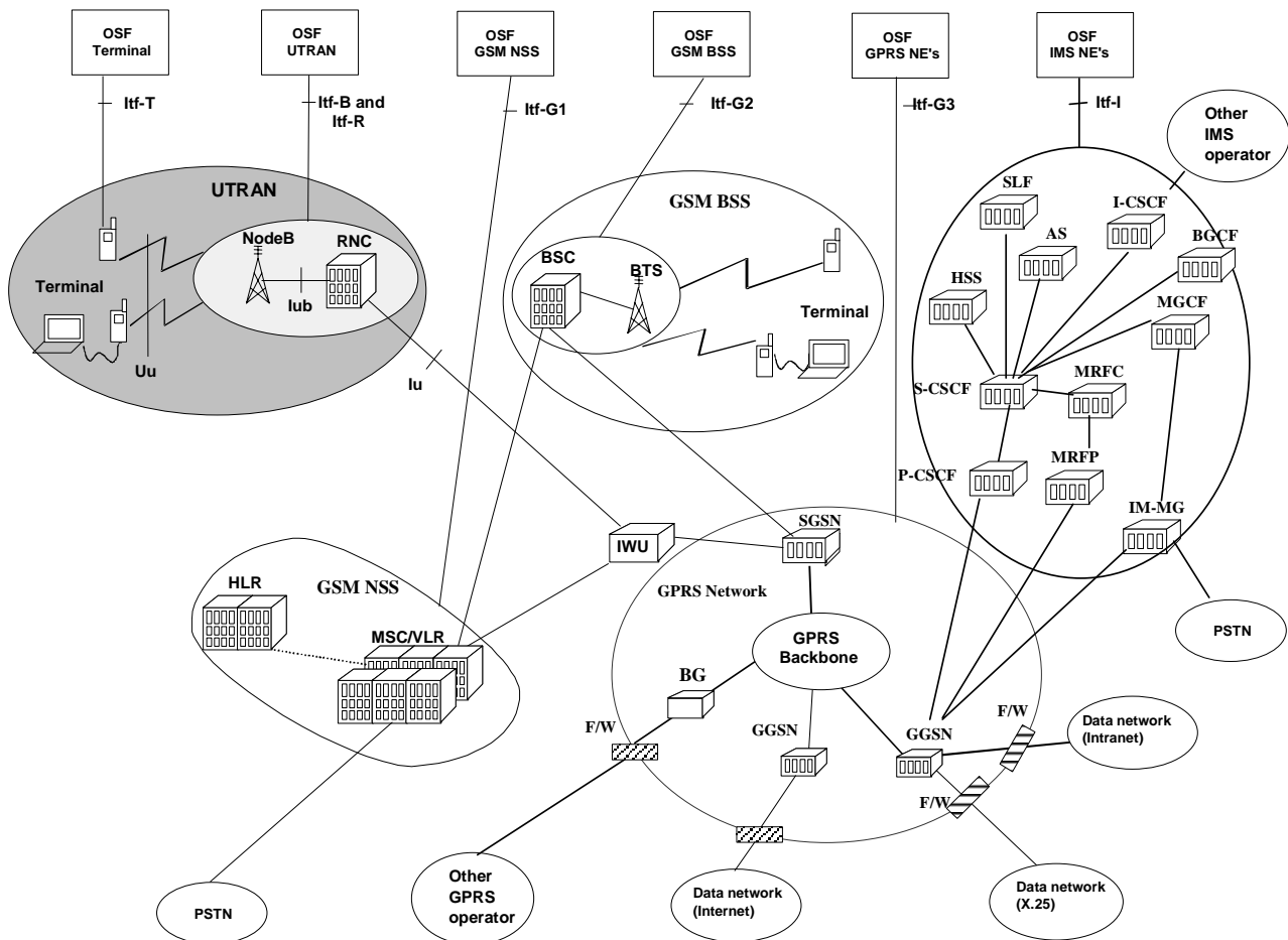
Figure B.1: Overview of a UMTS Network, showing management interfaces and management areas
