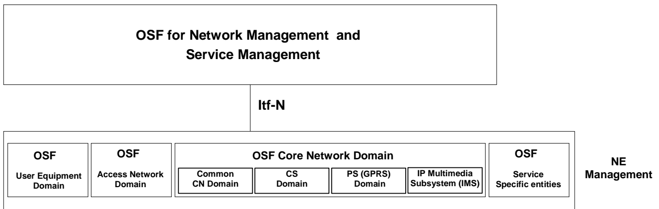
Figure 7.2: Overview of UMTS Telecom Management Domains and Itf-N
