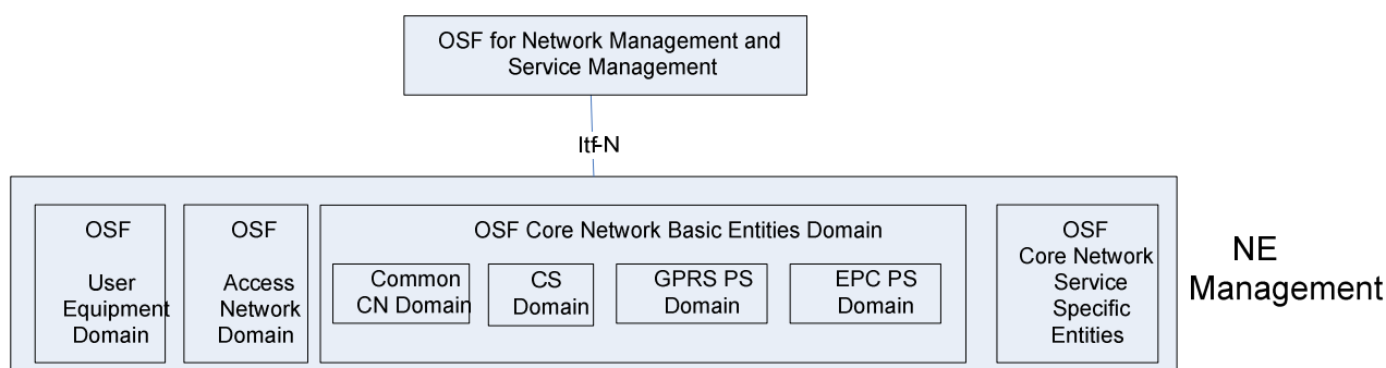
Figure 7.3.2.1: Overview of 3GPP Telecom Management Domains and Irf-N
