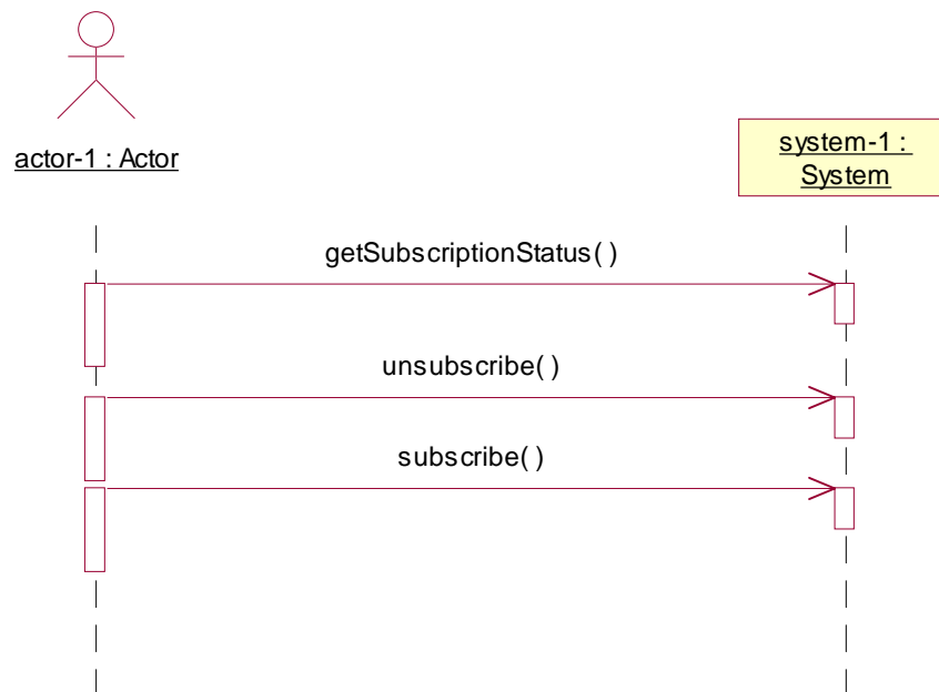
Figure 7: Interaction diagram for Heartbeat
