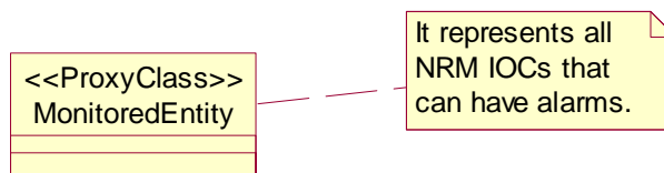
<<ProxyClass>> Notation
