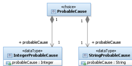
Figure 5.3.6.2-2: Operations model element example using «choice» notation
