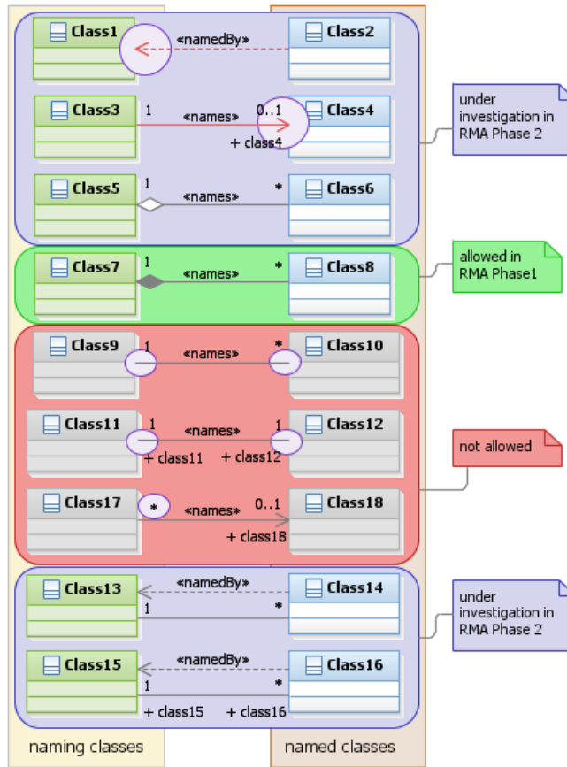
Figure D-1: Various forms of naming stereotypes
