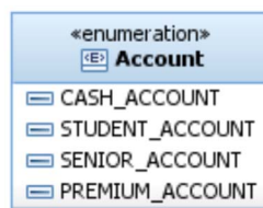
Figure 5.3.5.2-1: <<enumeration>> notation
