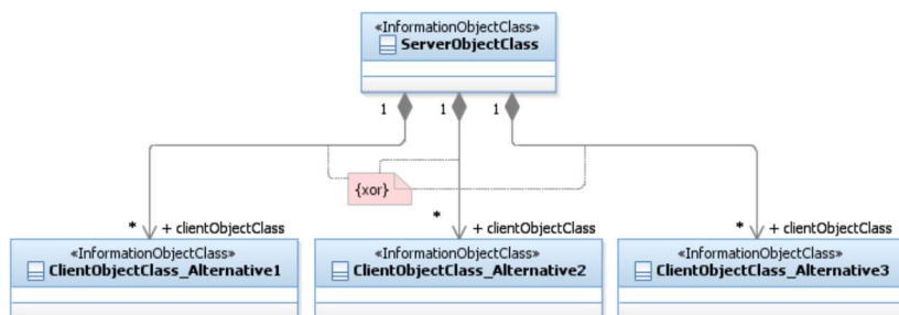
Figure 5.2.10.2-1: {xor} notation
