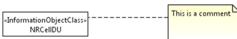
Figure 5.2.7.2-1: Comment notation
