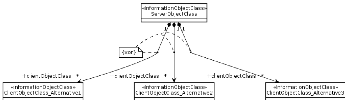
Figure 5.2.10.2-1: {xor} notation
