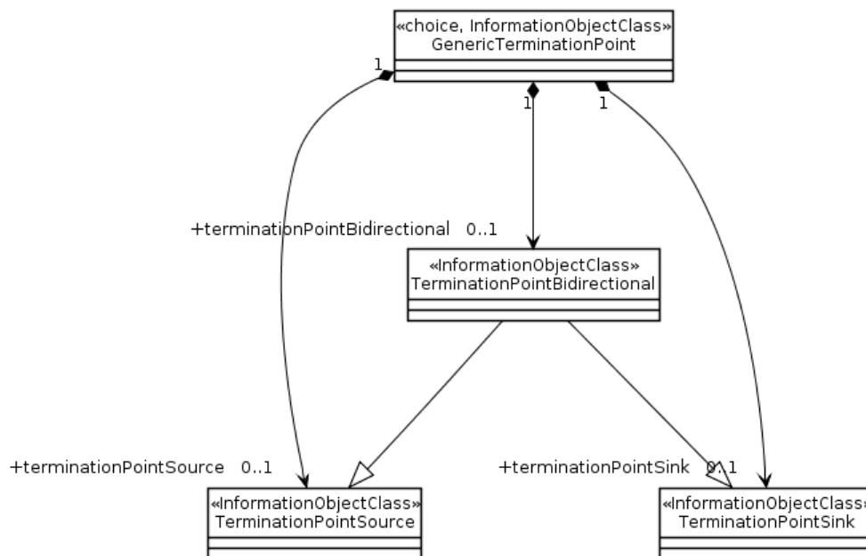
Figure 5.3.6.2-3: Sink/source/bidirectional termination points example using «choice» notation
