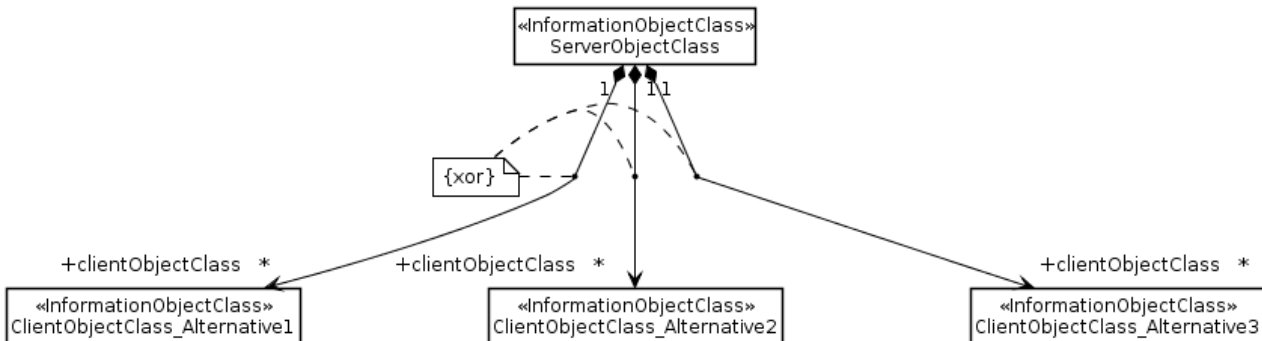
Figure 5.2.10.2-1: {xor} notation
