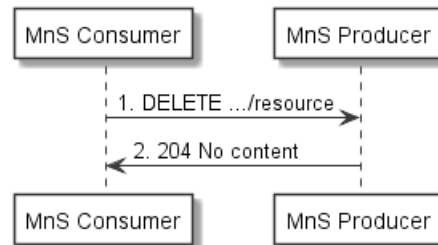
Figure 5.4-1: Flow for deleting a resource
