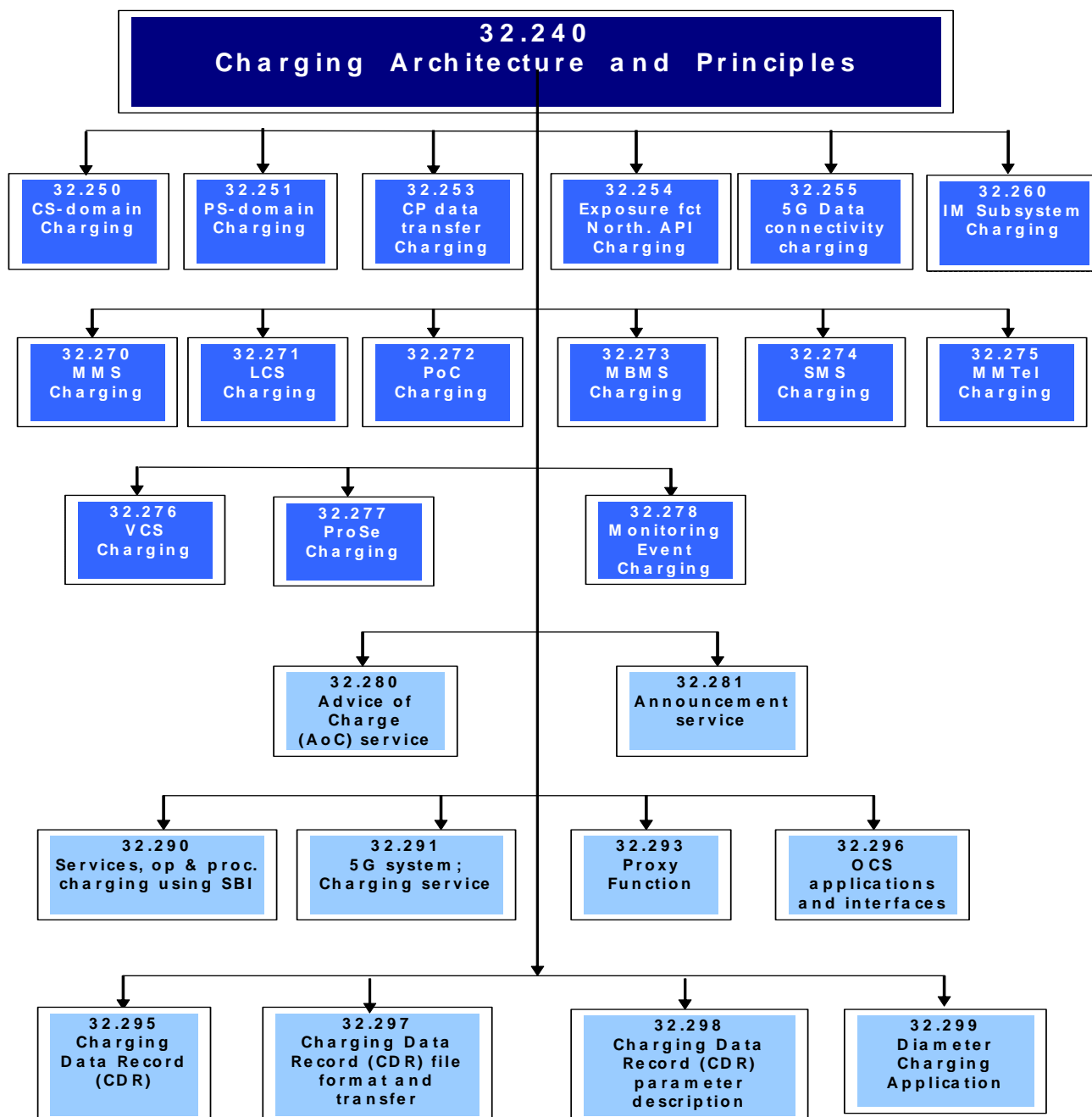
Figure 1.1: Charging specifications structure
