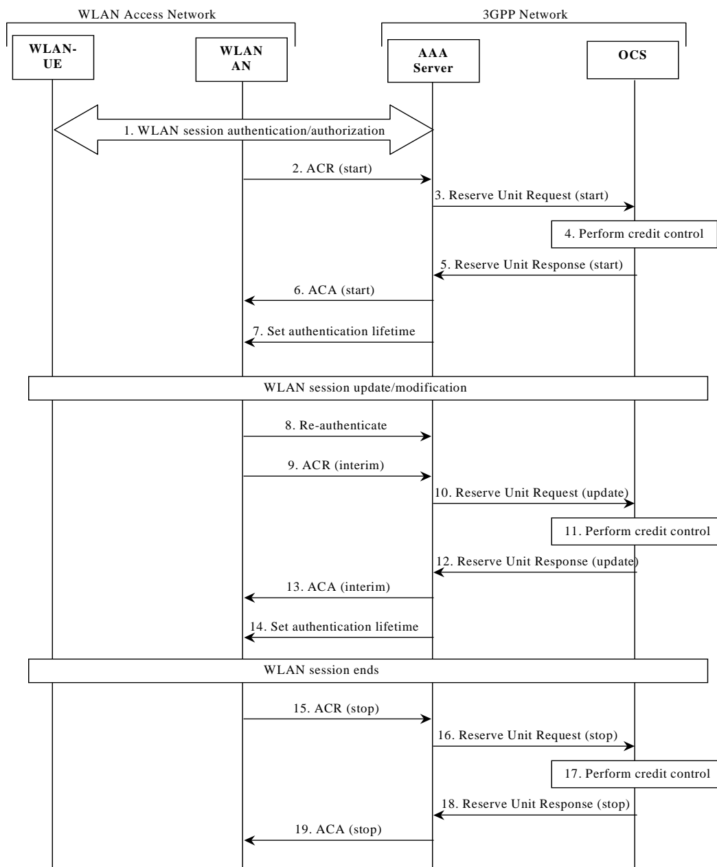
Figure 5.3.2.2: Message Sequence Chart for WLAN session when WLAN AN support Accounting
