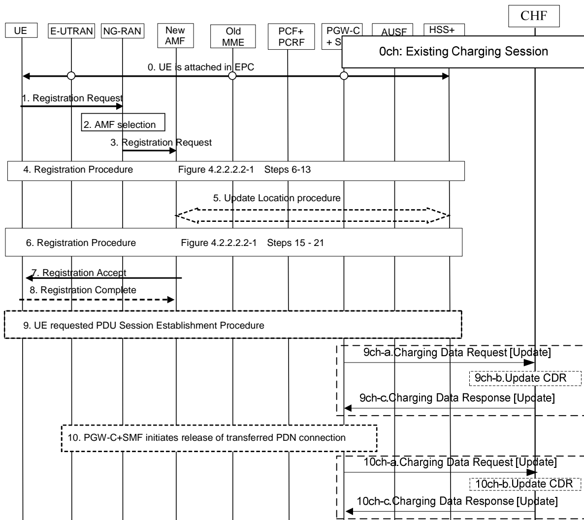
Figure 5.2.2.11.5.1: EPS to 5GS mobility without N26
