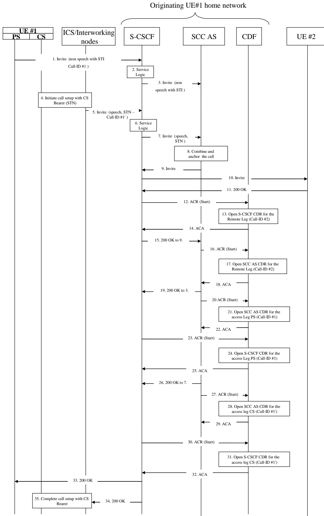
Figure 5.2.2.1.13.2-1: Message Sequence Chart UE originating call
