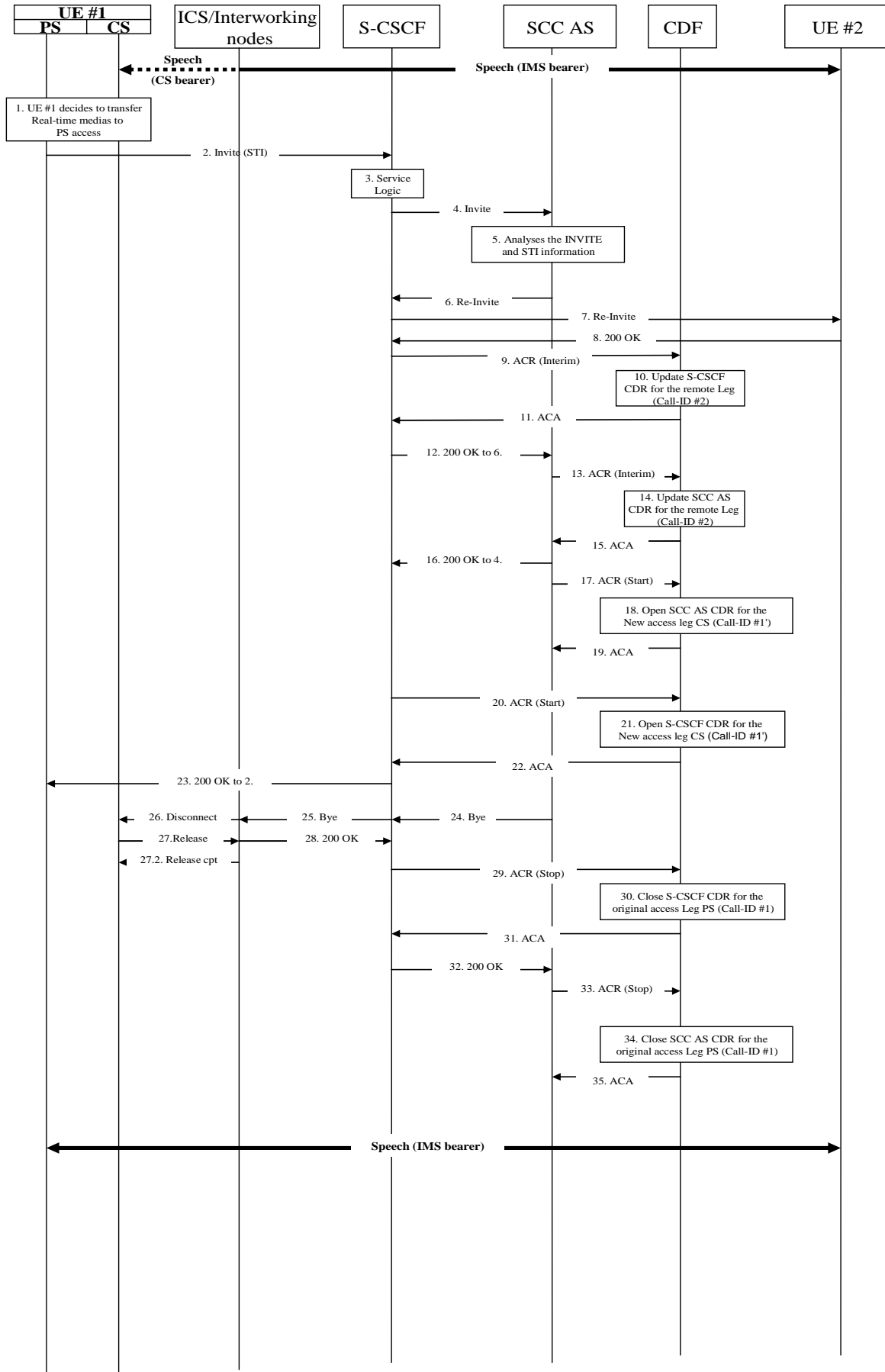
Figure 5.2.2.1.13.6-1: Message Sequence Chart UE Domain Transfer CS access to PS access.
