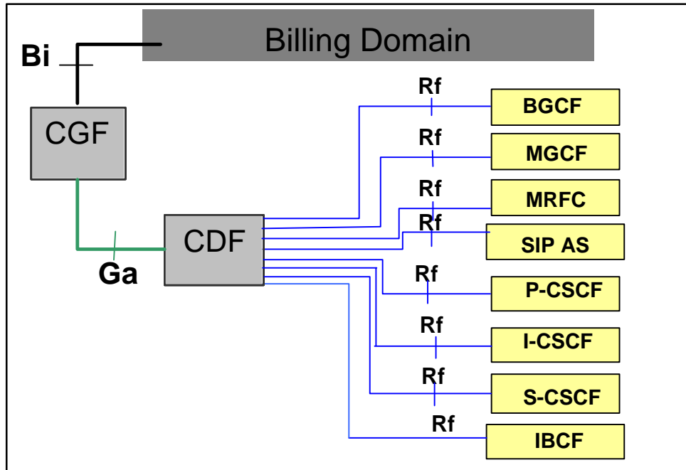
Figure 4.2: IMS offline charging architecture
