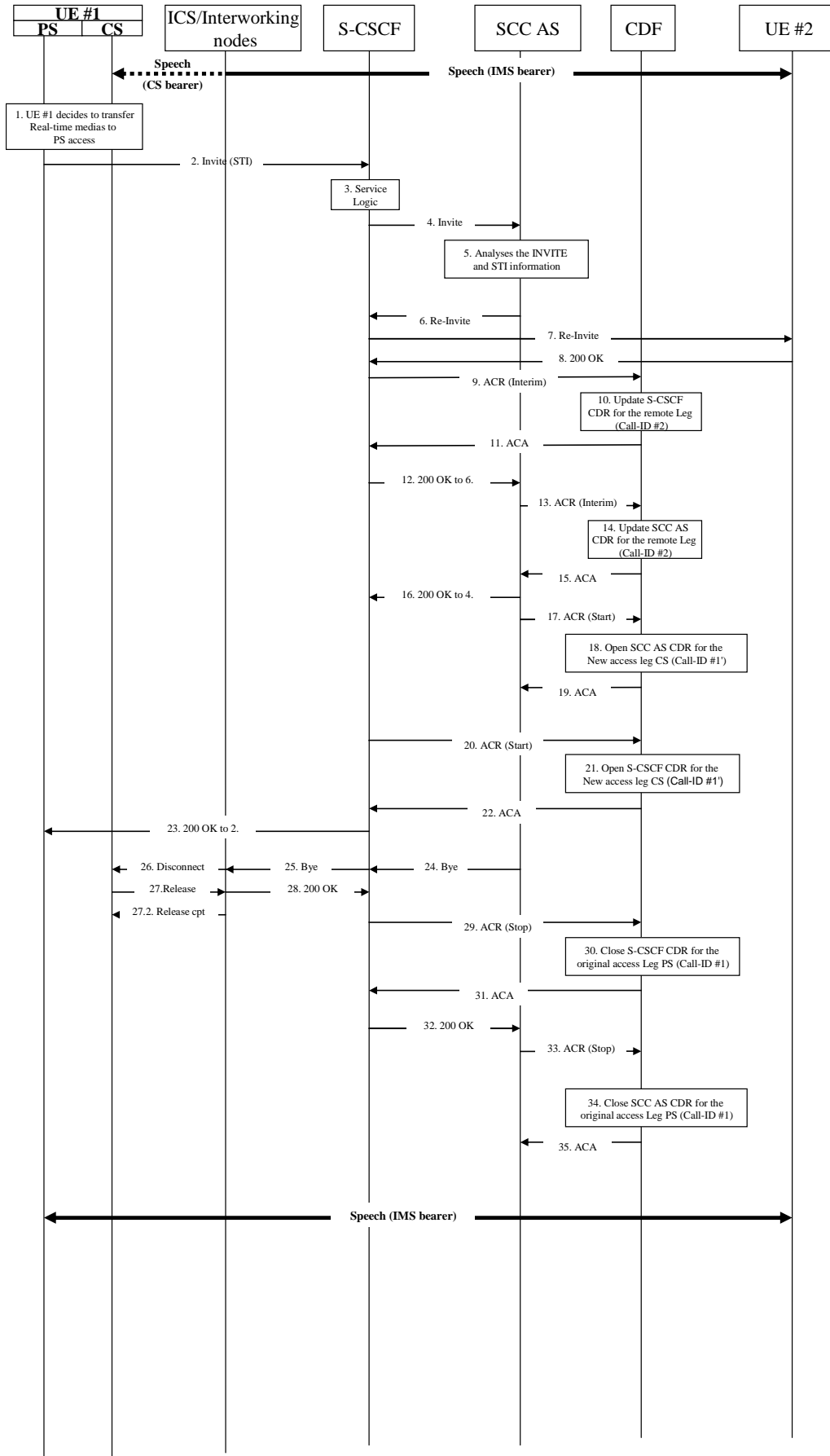
Figure 5.2.2.1.13.6-1: Message Sequence Chart UE Domain Transfer CS access to PS access.
