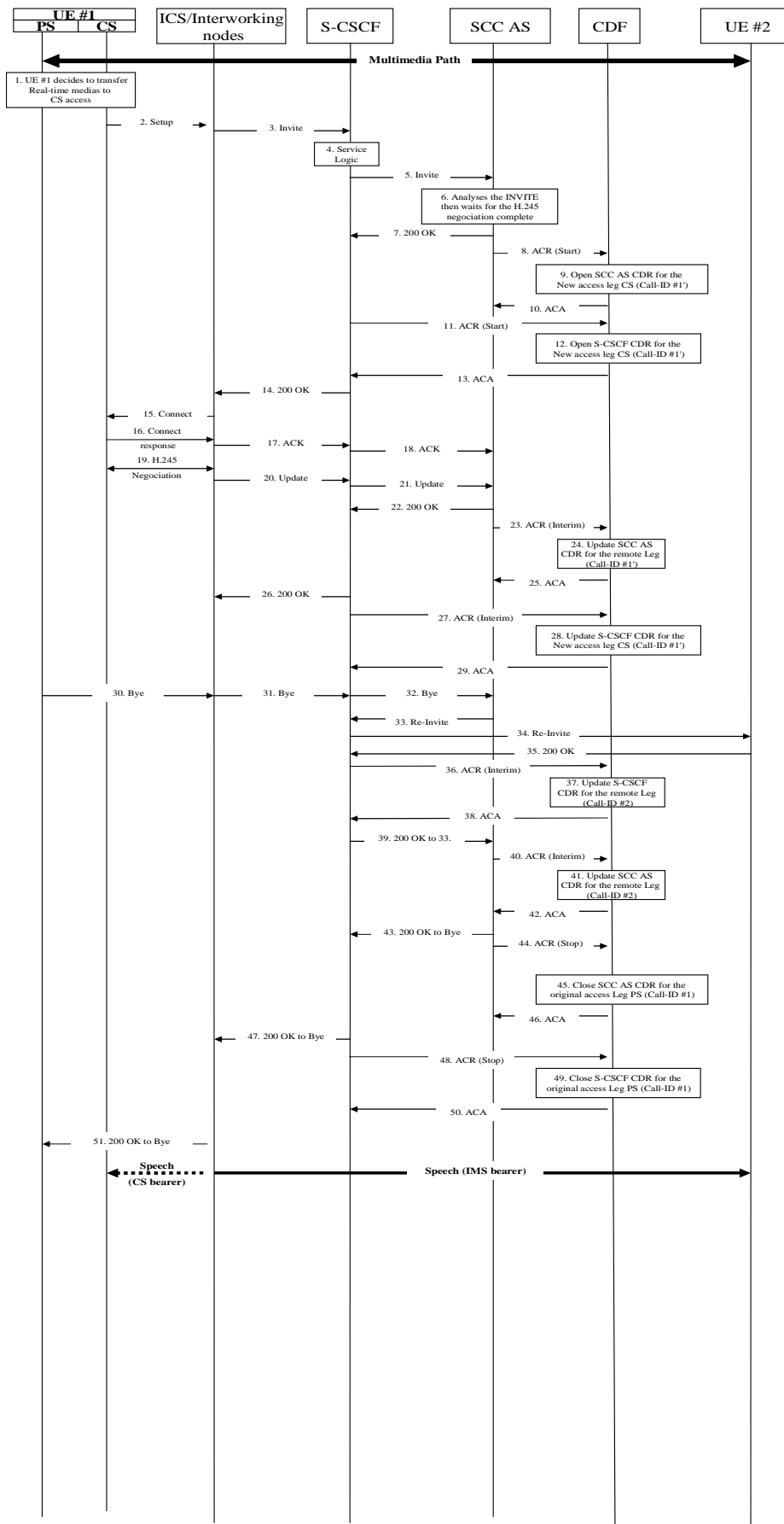
Figure 5.2.2.1.13.5-1: Message Sequence Chart UE Domain Transfer PS access to CS access.
