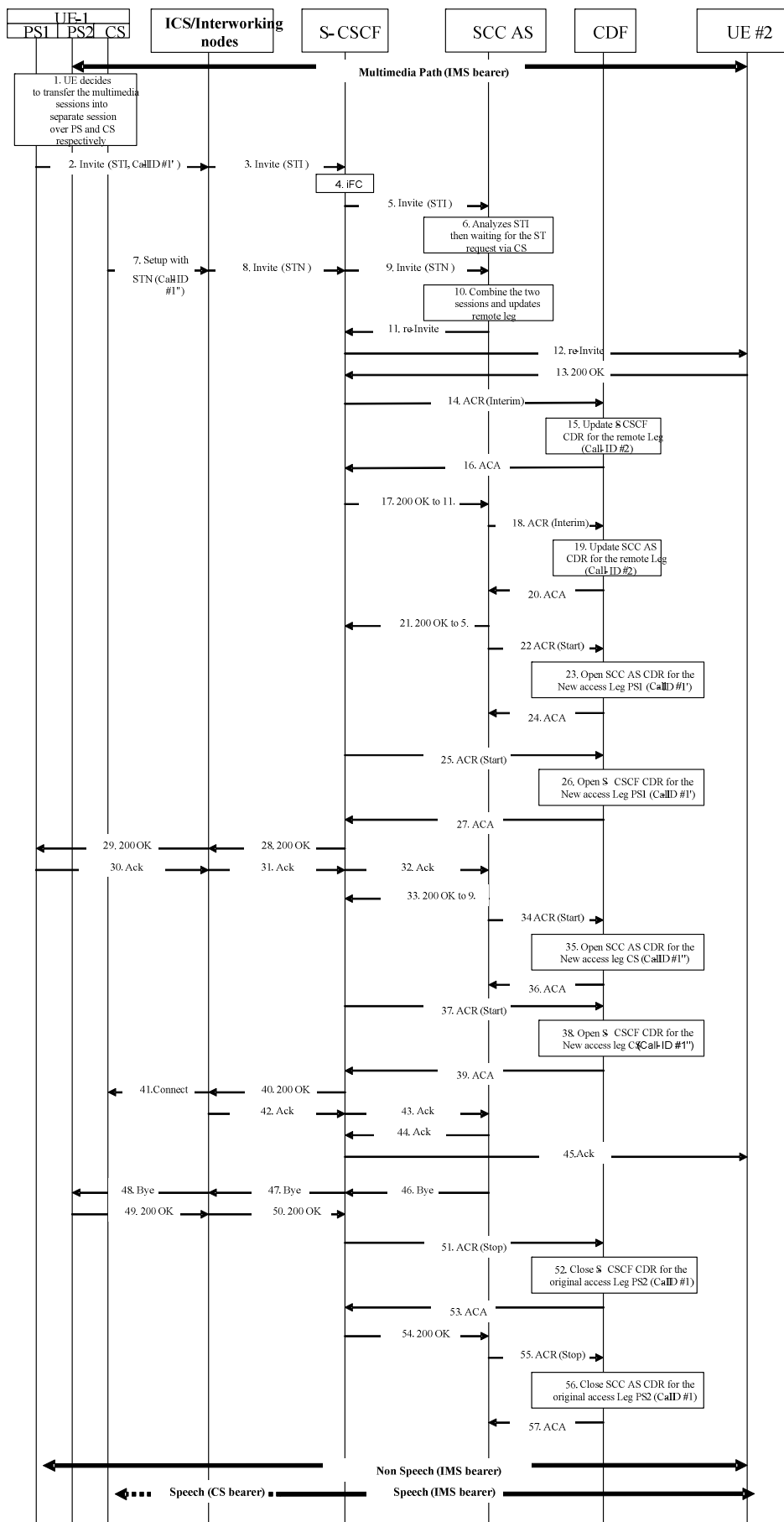
Figure 5.2.2.1.13.7-1: Message Sequence Chart UE Domain Transfer PS2 access to PS1 and CS access.
