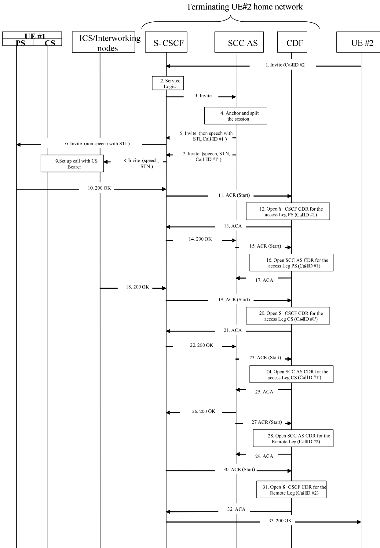
Figure 5.2.2.1.13.4-1: Message Sequence Chart UE terminating call
