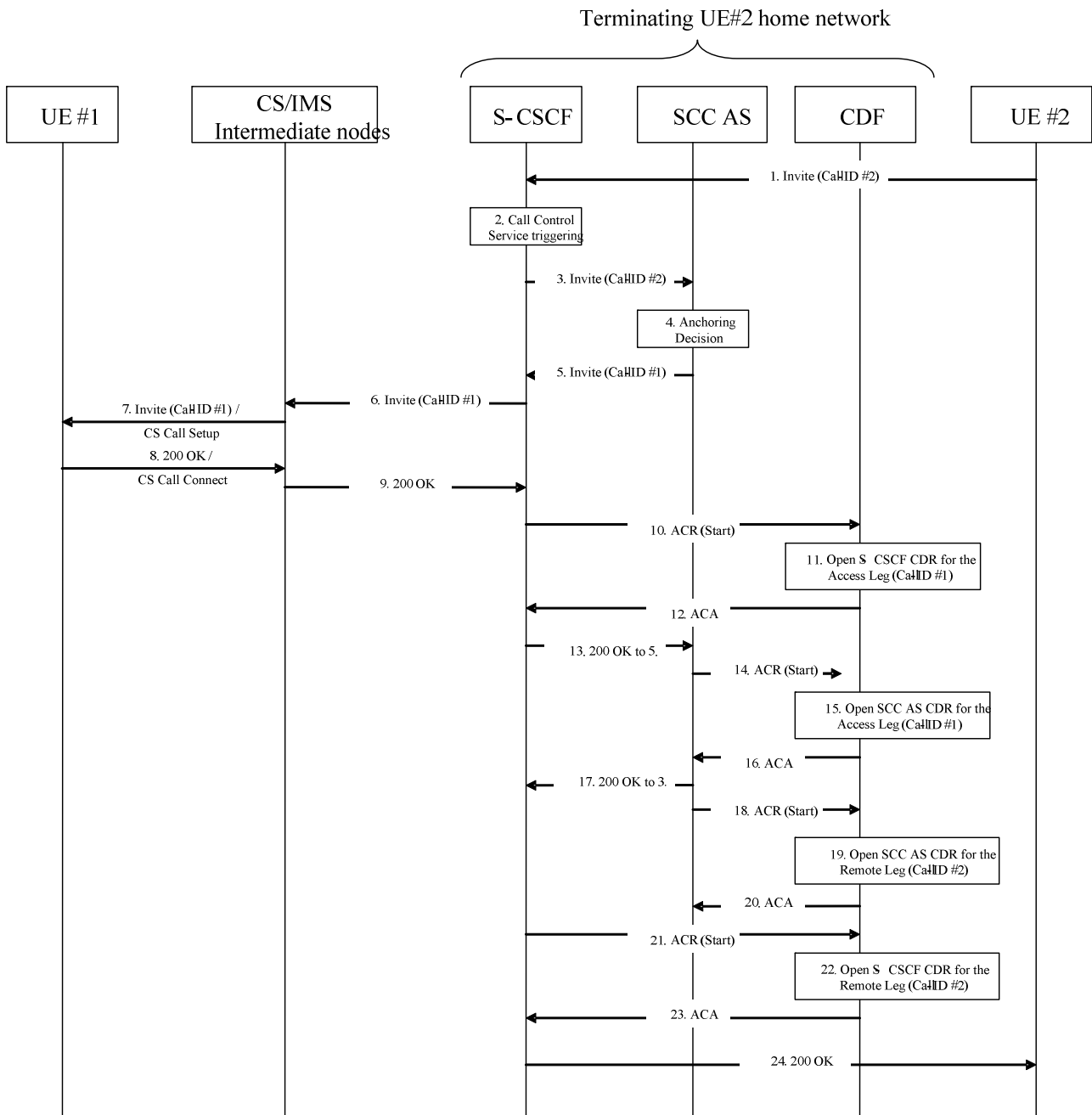
Figure 5.2.2.1.13.3-1: Message Sequence Chart UE terminating call
