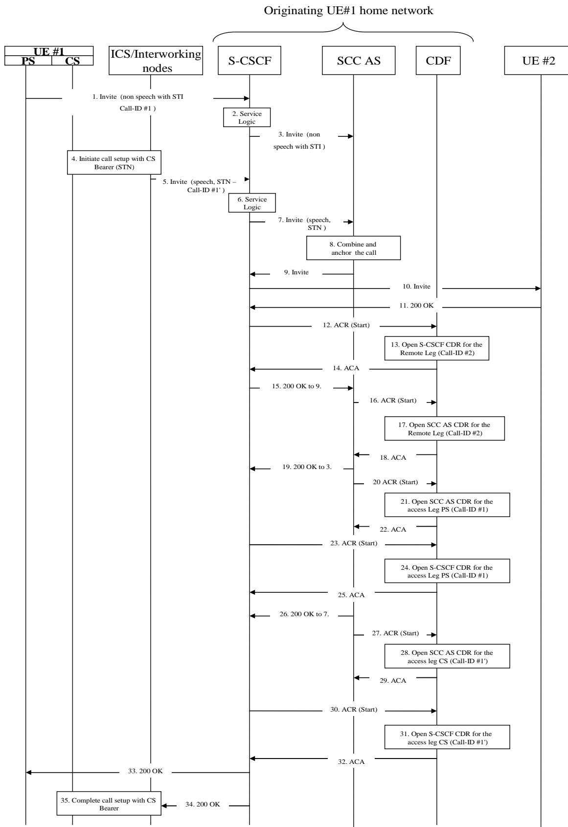
Figure 5.2.2.1.13.2-1: Message Sequence Chart UE originating call
