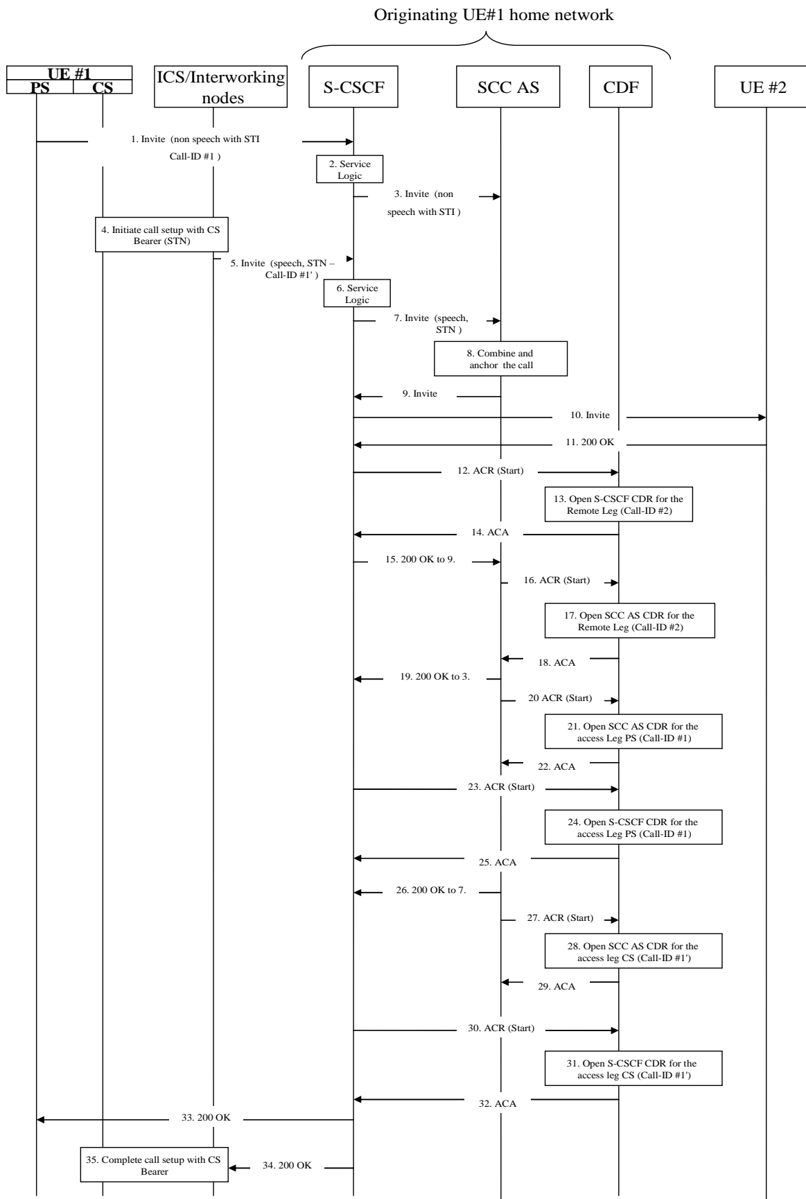
Figure 5.2.2.1.13.2-1: Message Sequence Chart UE originating call
