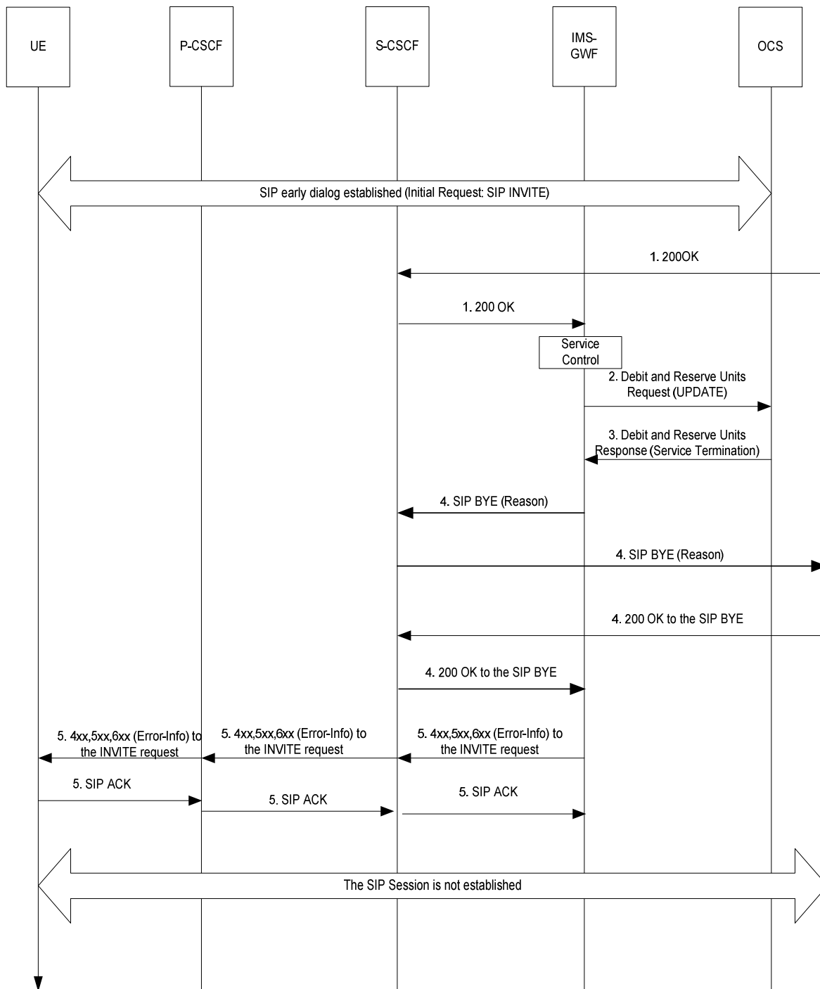
Figure B.2.1: Service Termination triggered by the 200OK response to the initial INVITE
