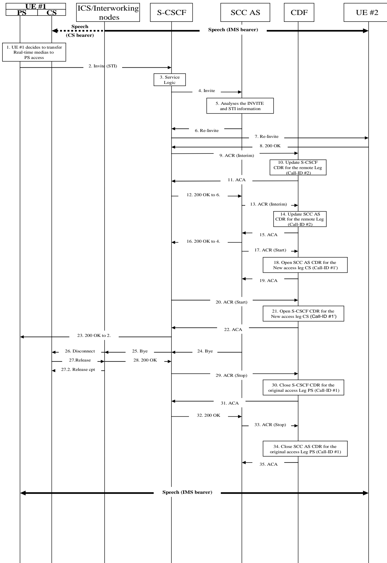
Figure 5.2.2.1.13.6-1: Message Sequence Chart UE Domain Transfer CS access to PS access.
