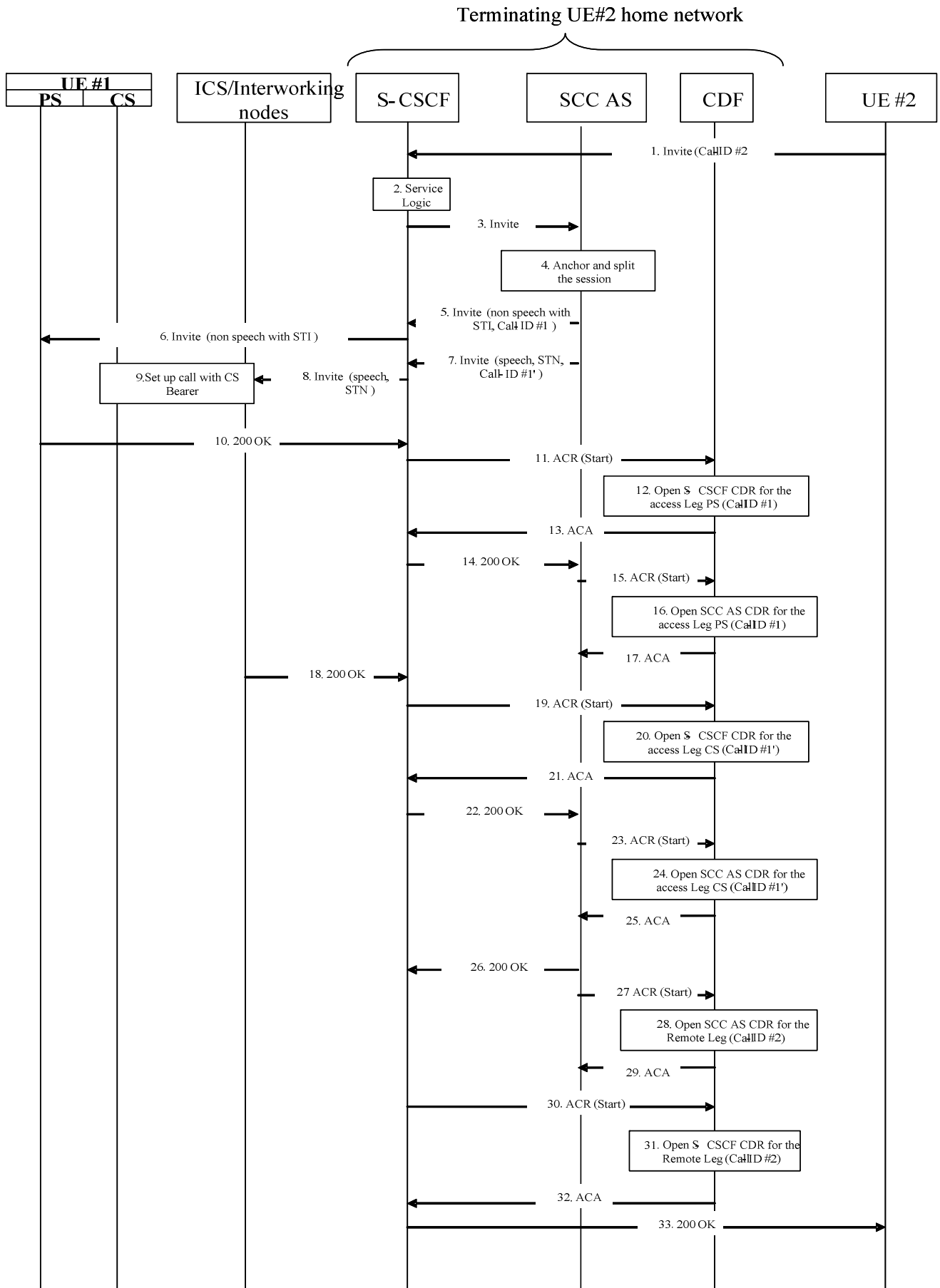
Figure 5.2.2.1.13.4-1: Message Sequence Chart UE terminating call
