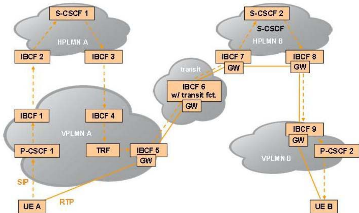
Figure 5.1.7: Signalling and media flows in a Roaming Architecture for Voice over IMS with Local Breakout (Example)
