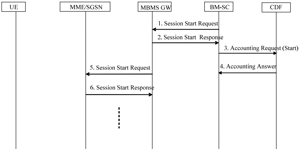
Figure 5.2.2.1.2A: Rf interaction during Broadcast Session Start Procedure for a broadcast bearer
