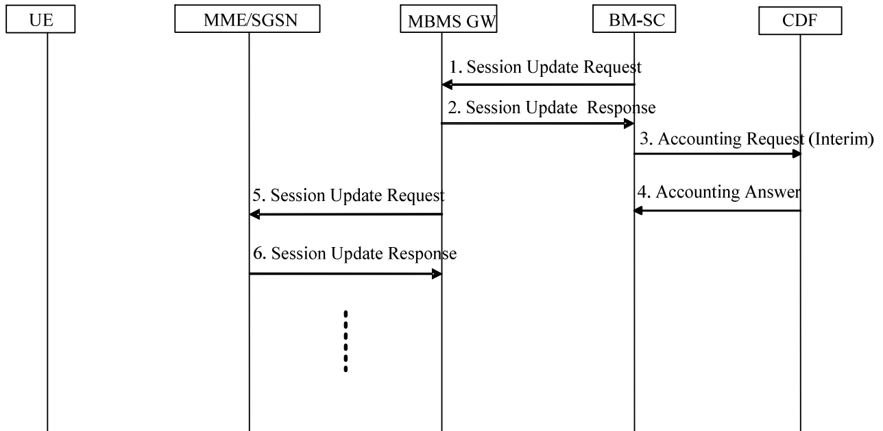
Figure 5.2.2.1.5: Rf interaction during Broadcast Session Update Procedure for a broadcast bearer
