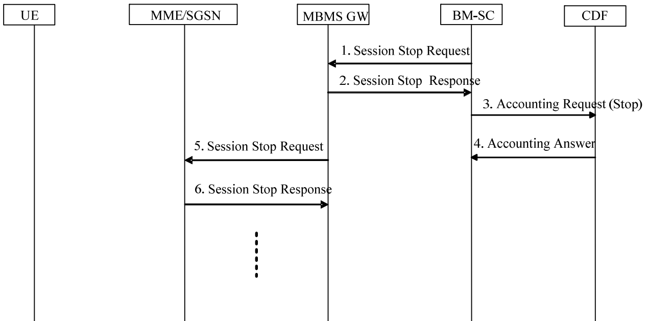
Figure 5.2.2.1.3A: Rf interaction during MBMS Session Stop procedure for a broadcast bearer
