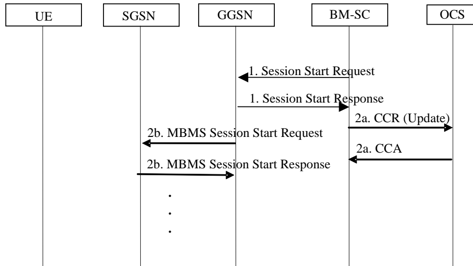
Figure 5.3.2.2.1: Ro interaction during MBMS Session Start procedure for a multicast bearer
