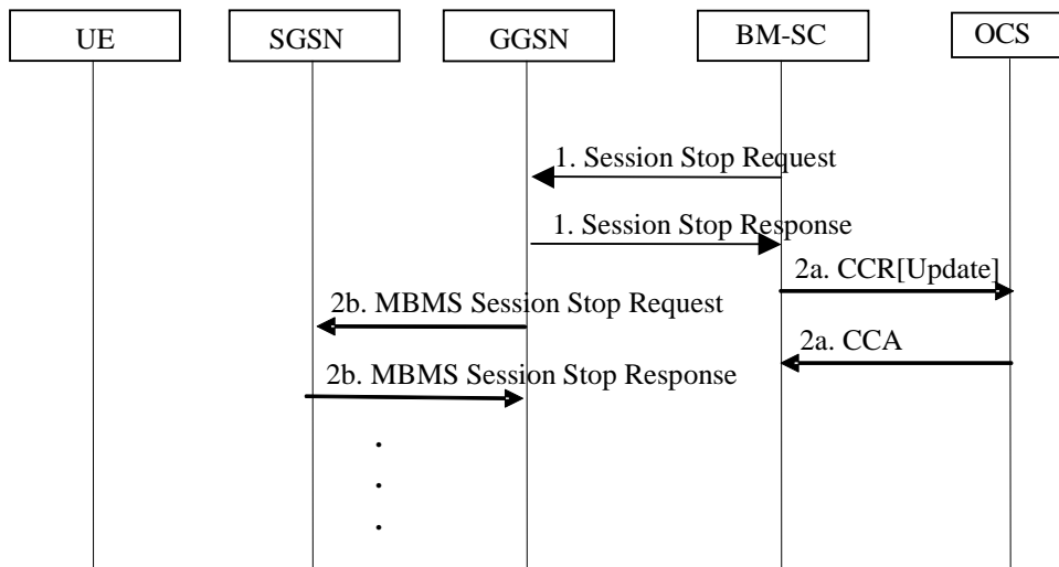
Figure 5.3.2.2.2.1: Ro interaction during MBMS Session Stop procedure for a multicast bearer
