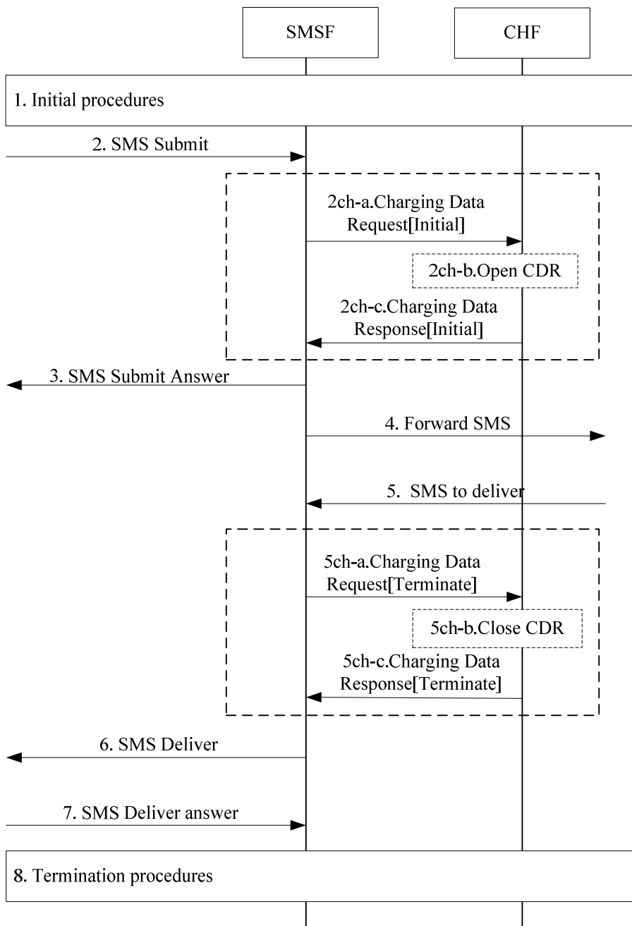
Figure 5.4.2.4.1: Converged charging SMS Submission using ECUR
