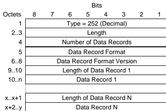
Figure 6.2.4.5.3.1: Data Record Packet IE
