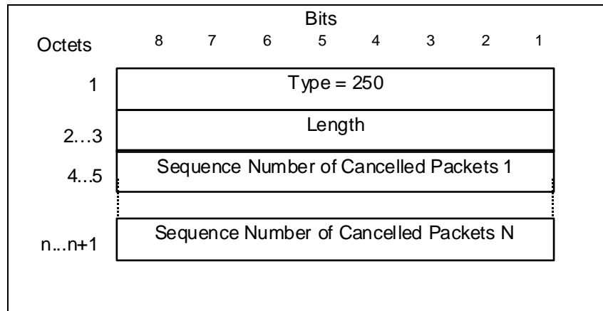
Figure 6.2.4.5.5.1: Sequence Numbers of Cancelled Packets IE
