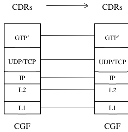
Figure 5.1.2.2.1: Protocol stack between CGFs
