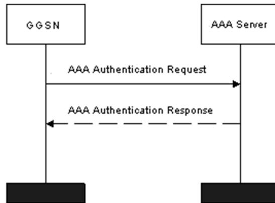
Figure: AAA authentication procedure initiated by GGSN
