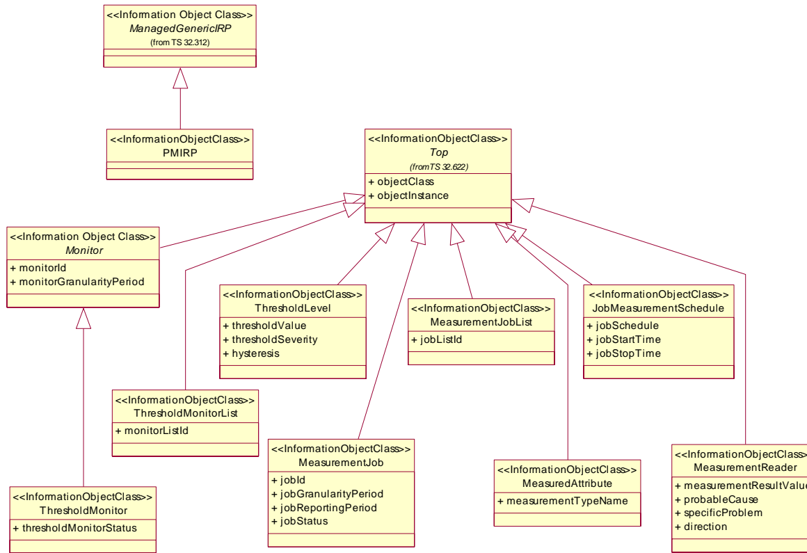
Figure 6.2.2: Information Object Class Inheritance UML Diagram
