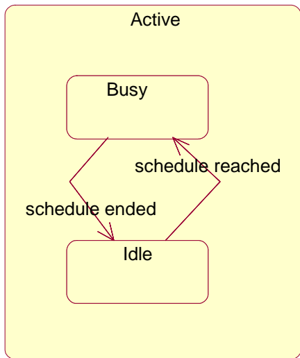
Figure 6.3.1.3.2: SubState Diagram of Active
