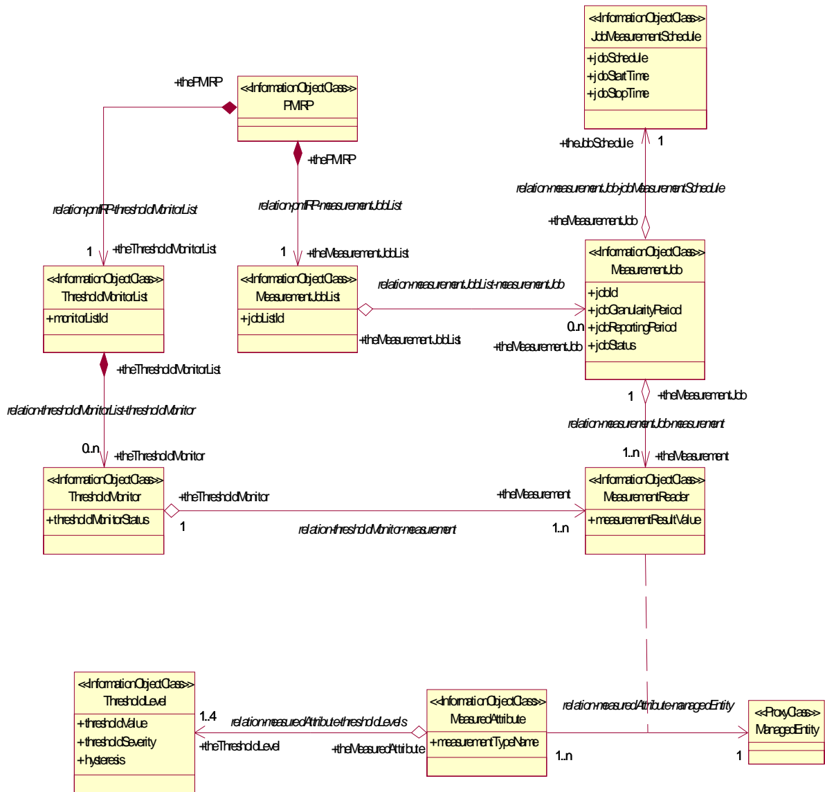
Figure 6.2.1(c): Information Object Class UML Diagram - Combined
