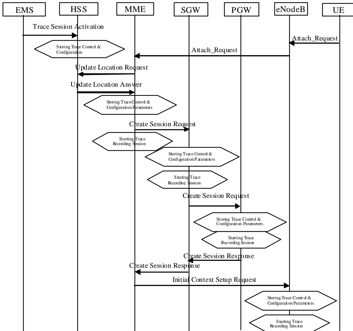
Figure 4.1.2.10.1: Trace Session activation procedure in EPC:
