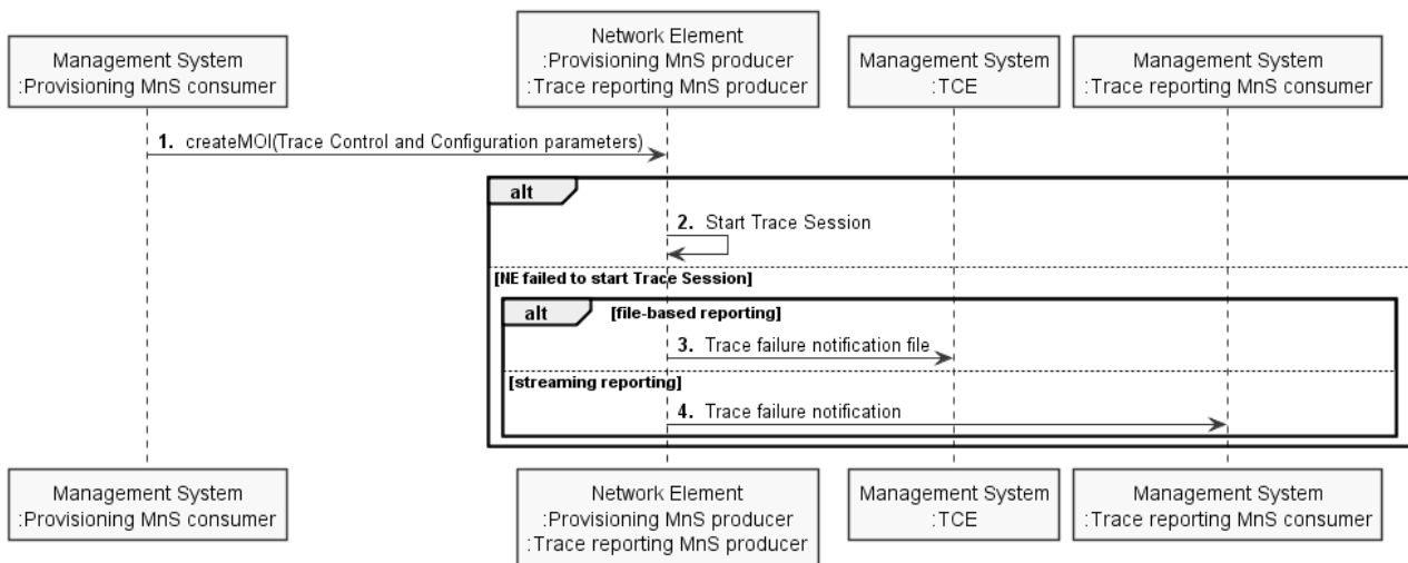
Figure 4.1.1.2-1: Overview of management activation for 5GS
