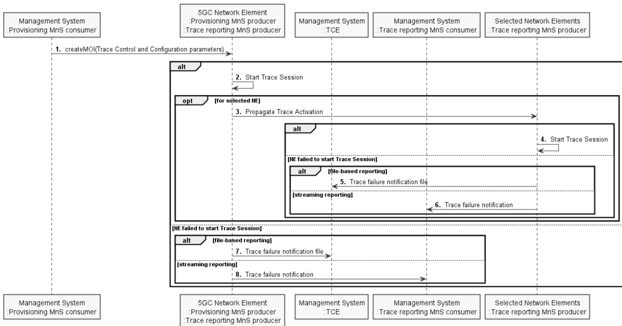
Figure 4.1.2.1.2-1: Overview of signaling activation for 5GS
