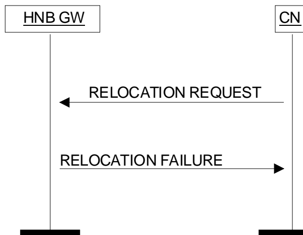
Figure 9 CSG UE Inbound Procedure: Unsuccessful Operation
