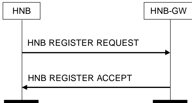
Figure 5 HNB Register Procedure: Successful Operation
