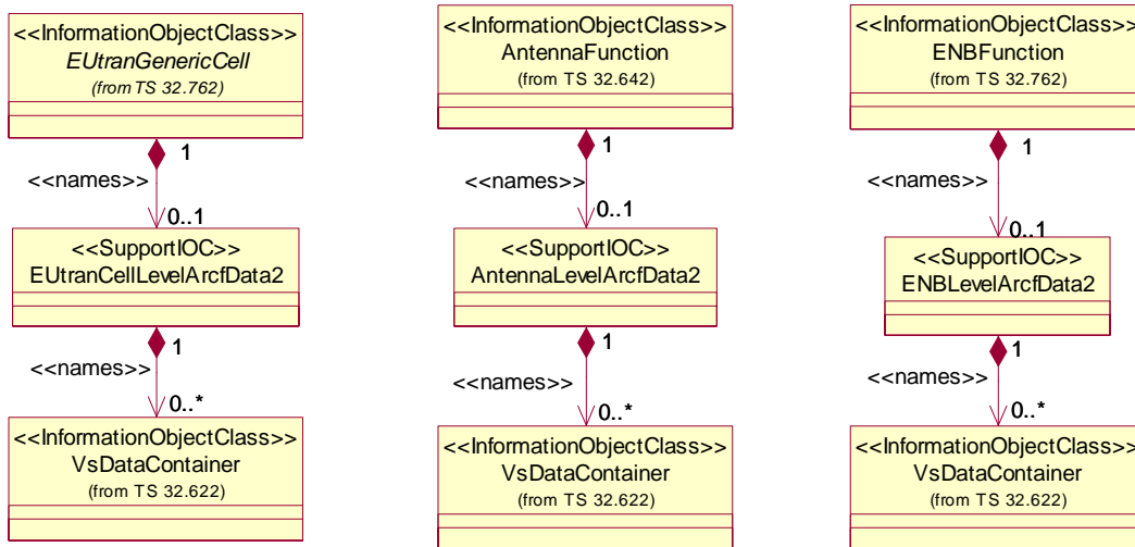
Figure 5.2.1-4: Definition of ARCF IOCs for usage of Bulk CM IRP
