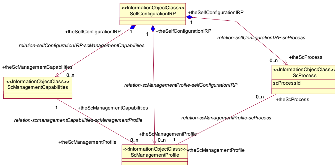
Figure 5.2.1-1: Self Configuration IRP Containment/Naming and Association diagram
