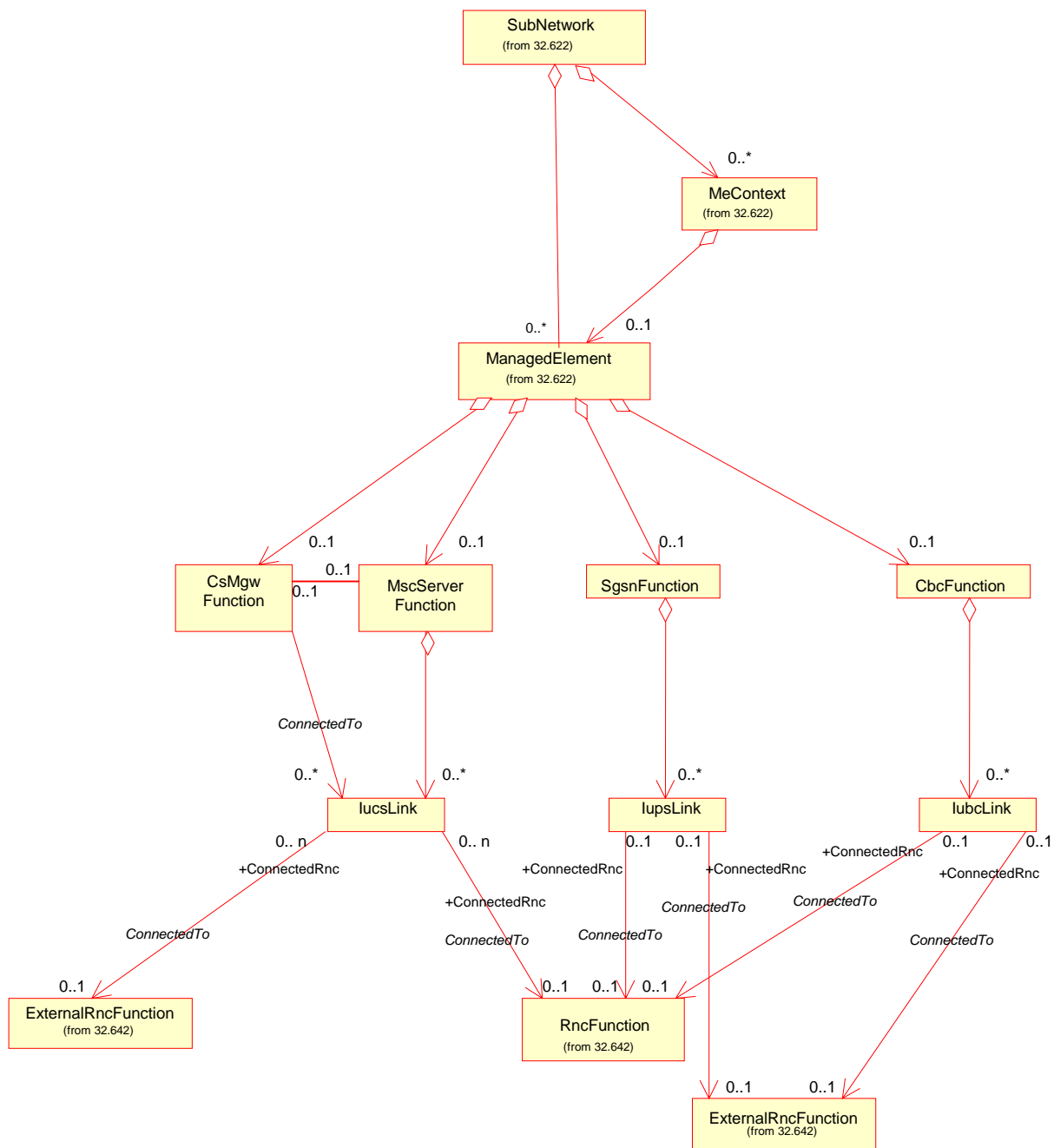
Figure 6.5: CN-UTRAN NRM Containment/Naming and Association diagram 3
