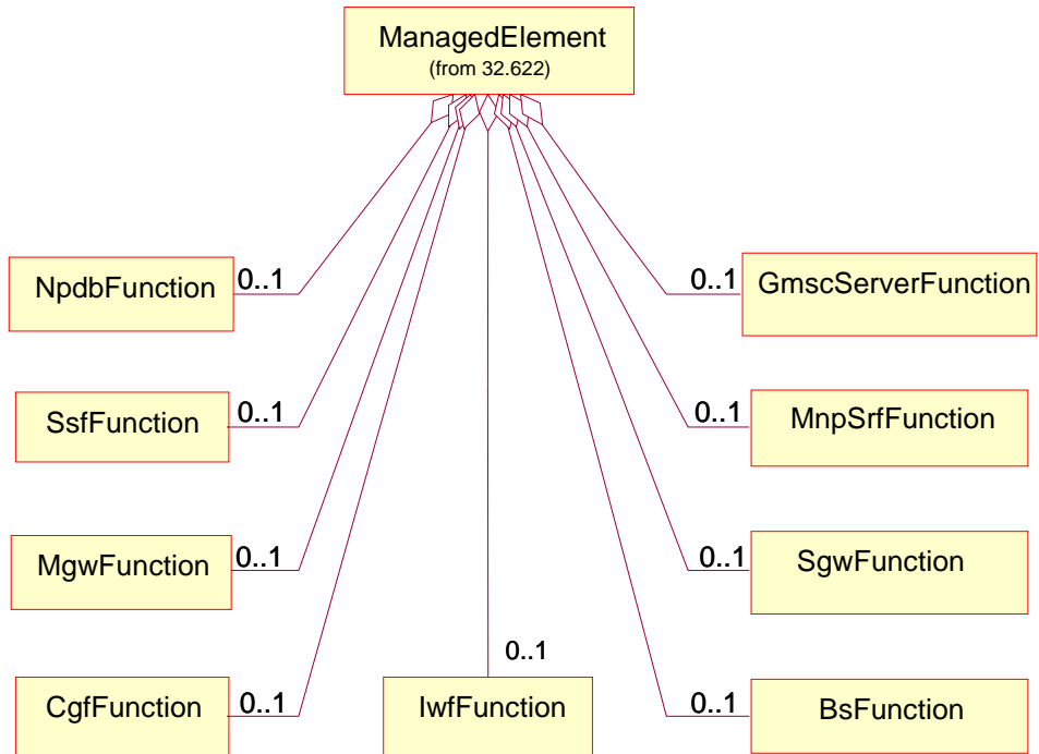
Figure 6.4: CN NRM Containment/Naming and Association diagram 2
