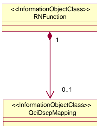
Figure 6.2.1.2a: E-UTRAN relaying view of E-UTRAN NRM
