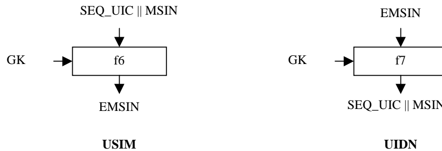
Figure A.1: Encryption and decryption of the permanent user identity
